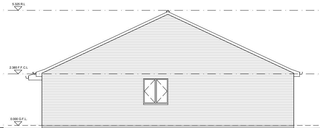
SIDE 2 ELEVATION
